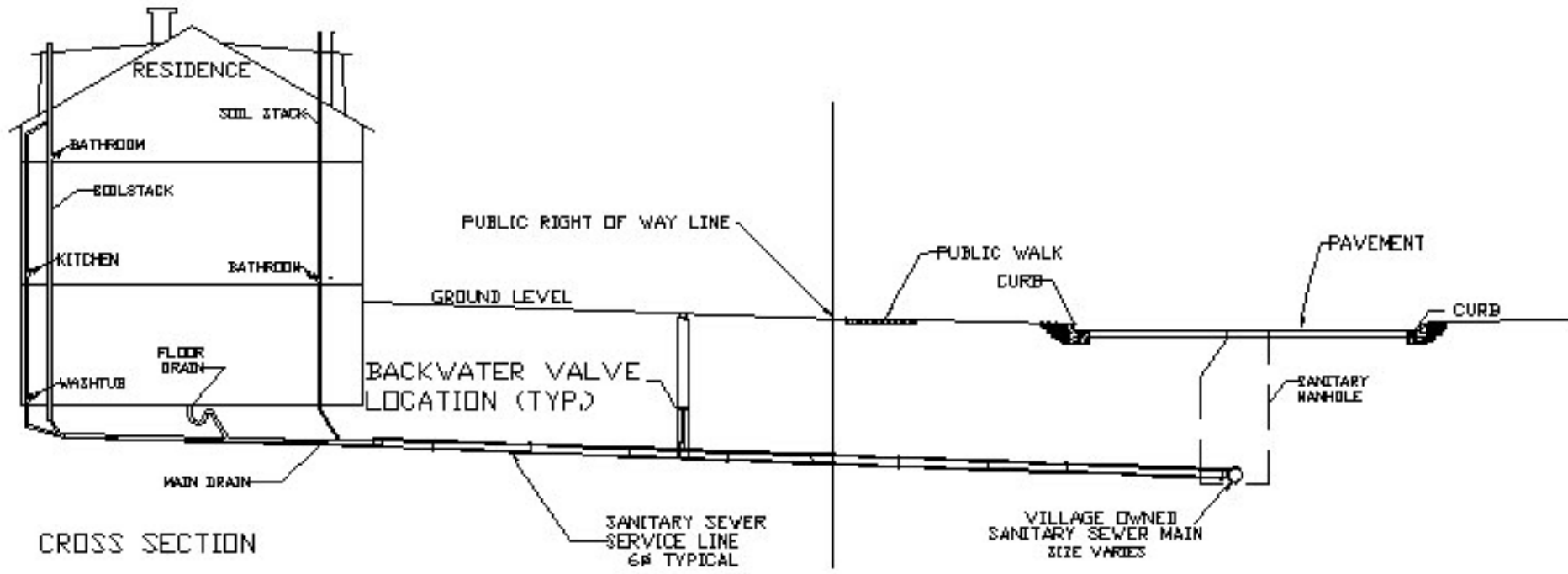
SANITARY SEWER SERVICE DIAGRAM SHOWING LOCATION OF BACKWATER VALVE
