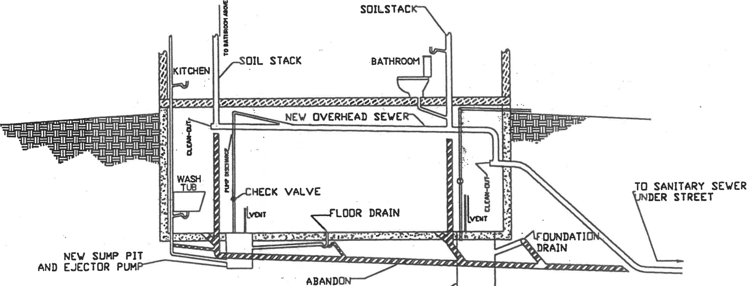
SECTION THRU BASEMENT SHOWING TYPICAL UNDER FOUNDATION SANITARY SEWER
