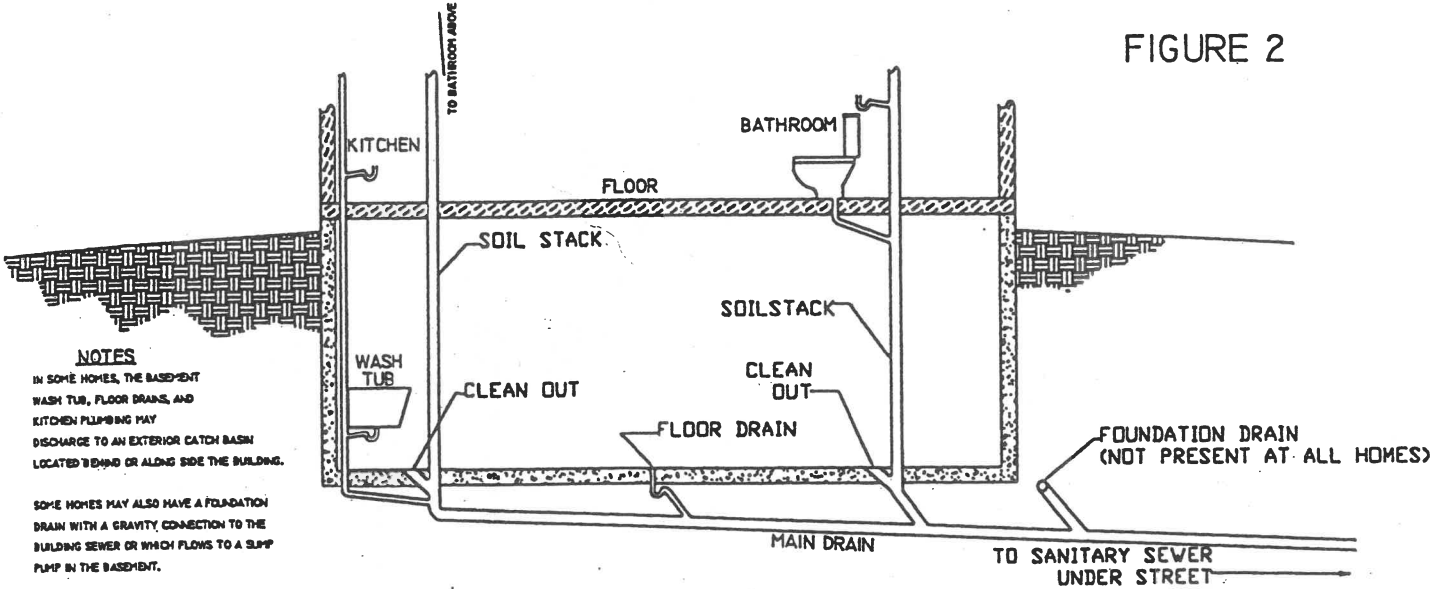
SECTION THRU BASEMENT SHOWING TYPICAL UNDER FOUNDATION SANITARY SEWER
